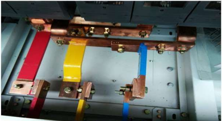
Bus Bar Connection
